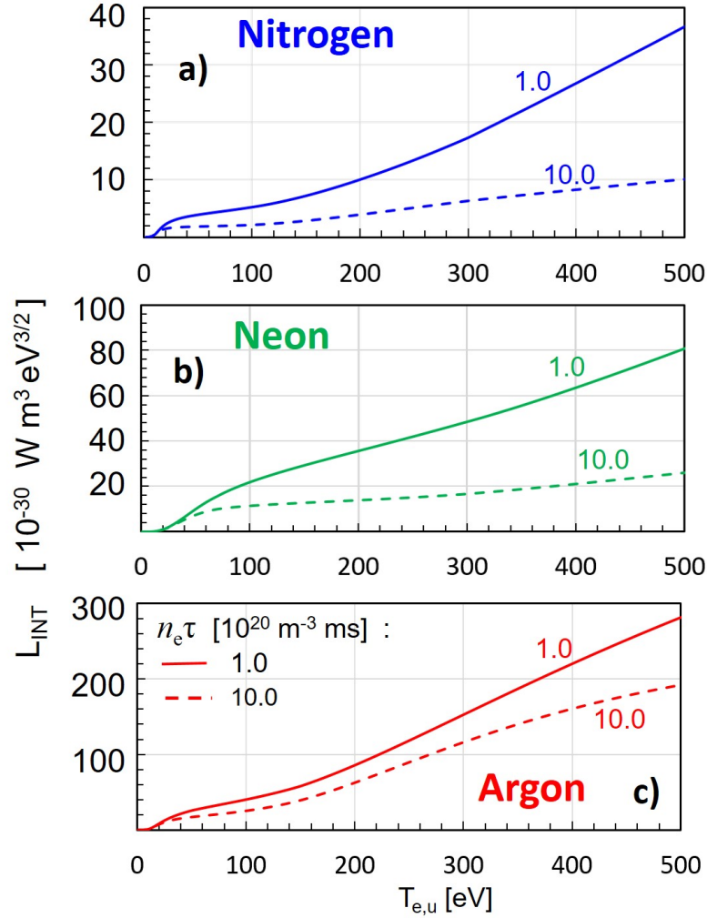
Fig. 2. L_{INT} as a function of T_{e,u} for \text{N}_2 , Ne and Ar and two values of the non-coronal parameter of n_e \tau : 1.0 \times 10^{20} \text{ m}^{-3} \text{ ms} and 10.0 \times 10^{20} \text{ m}^{-3} \text{ ms} .
