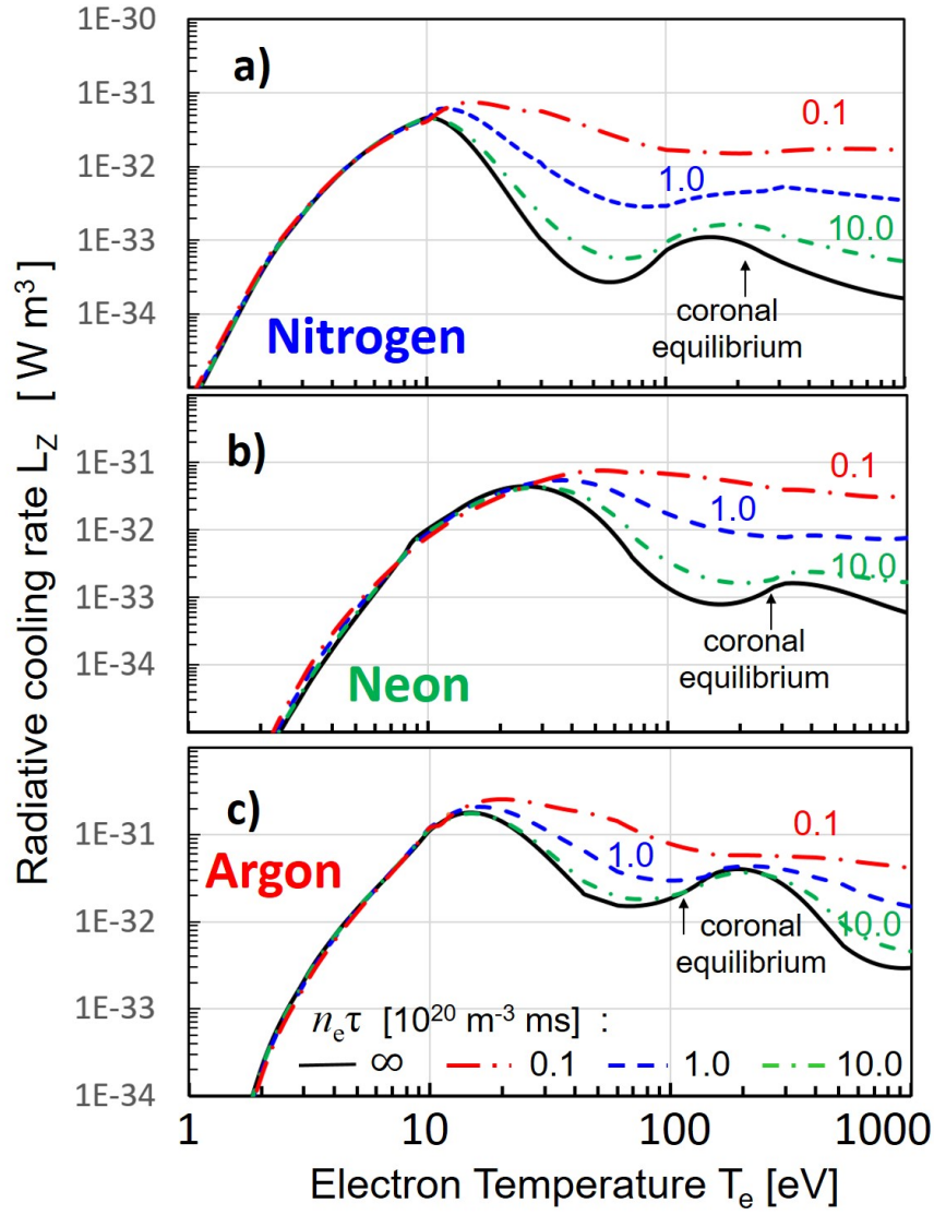
Fig. 1. The cooling rate coefficient L_Z for N 2 , Ne and Ar and several assumptions of n_e \tau : 0.1 \times 10^{20} \text{ m}^{-3} \text{ ms} , 1.0 \times 10^{20} \text{ m}^{-3} \text{ ms} and 10.0 \times 10^{20} \text{ m}^{-3} \text{ ms} .
